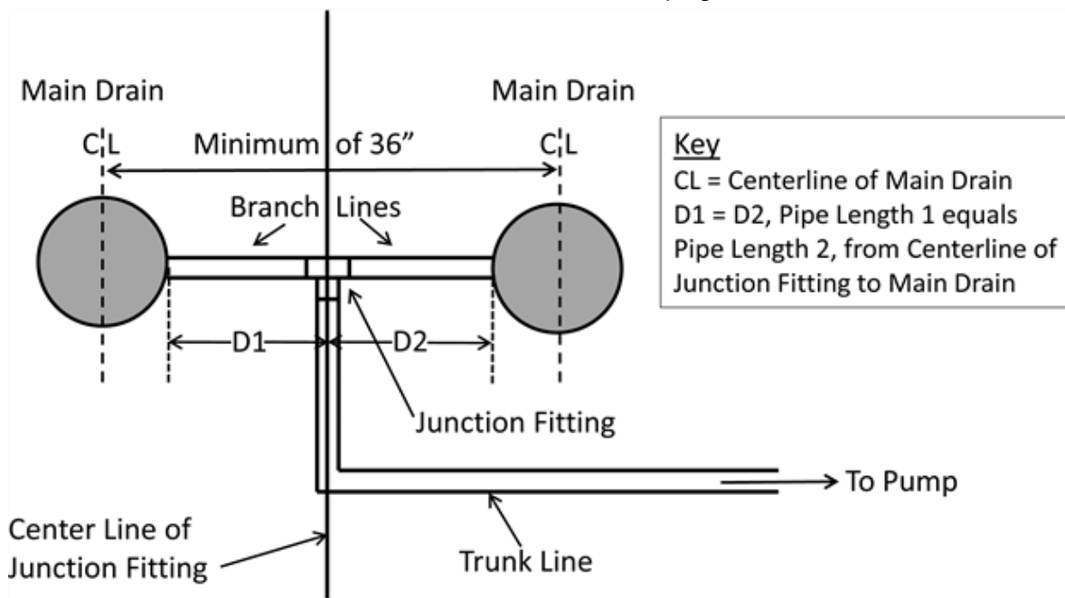
Figure 031.3 Main Drain Branch Line Piping Detail
