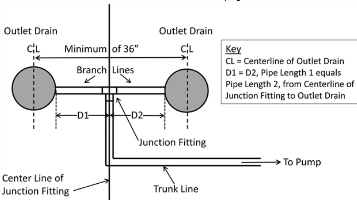
Outlet Drain Branch Line Piping Detail
