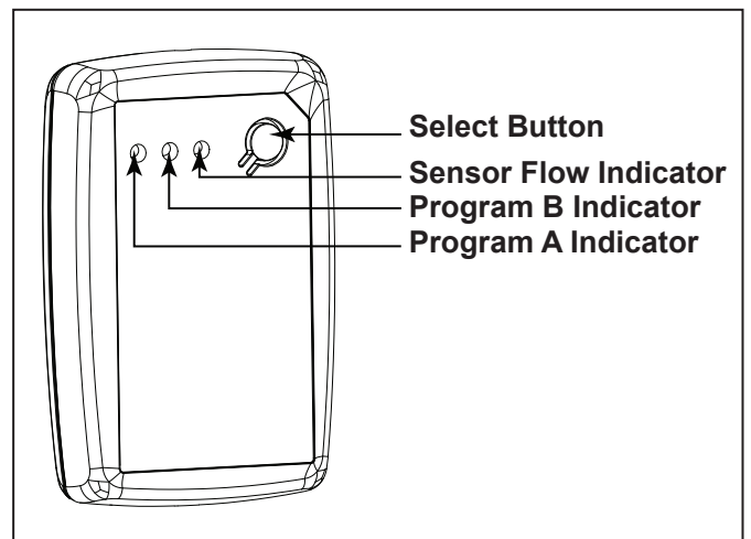
Figure 6. Tri-Sensor Interface Module
