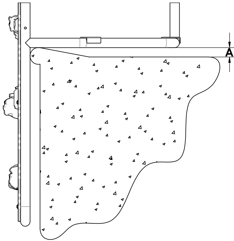
BULL NOSE COPING DIMENSION A REQUIRED
