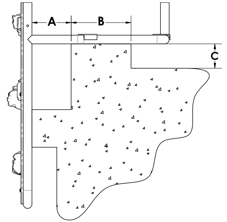
HAUNCH GUTTER DIMENSIONS A, B & C REQUIRED
