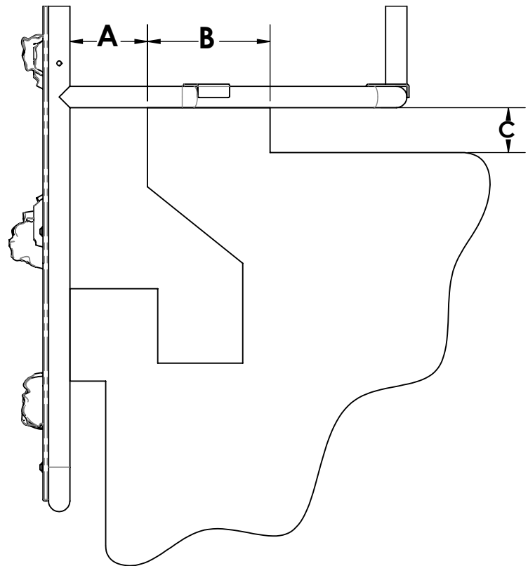
RECESSED GUTTER DIMENSIONS A, B & C REQUIRED
