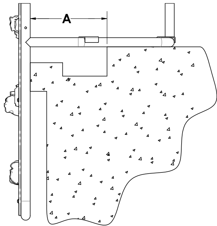
TROUGH GUTTER DIMENSION A REQUIRED
