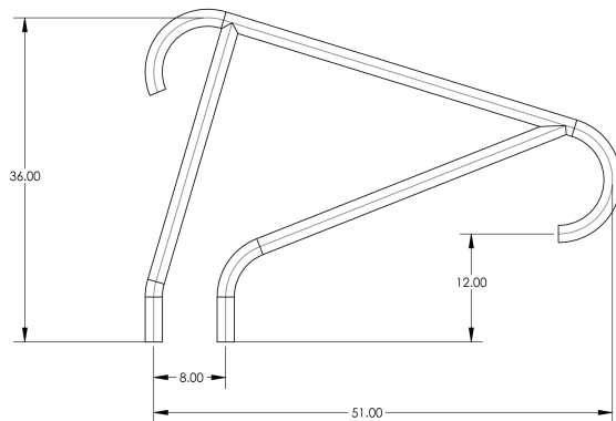
Deck-Mounted Stair Rail
