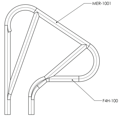
Overlay of MER-1001S and Figure 4 Hand Rail
