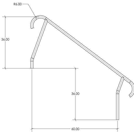
Deck-Mounted Stair Rail
