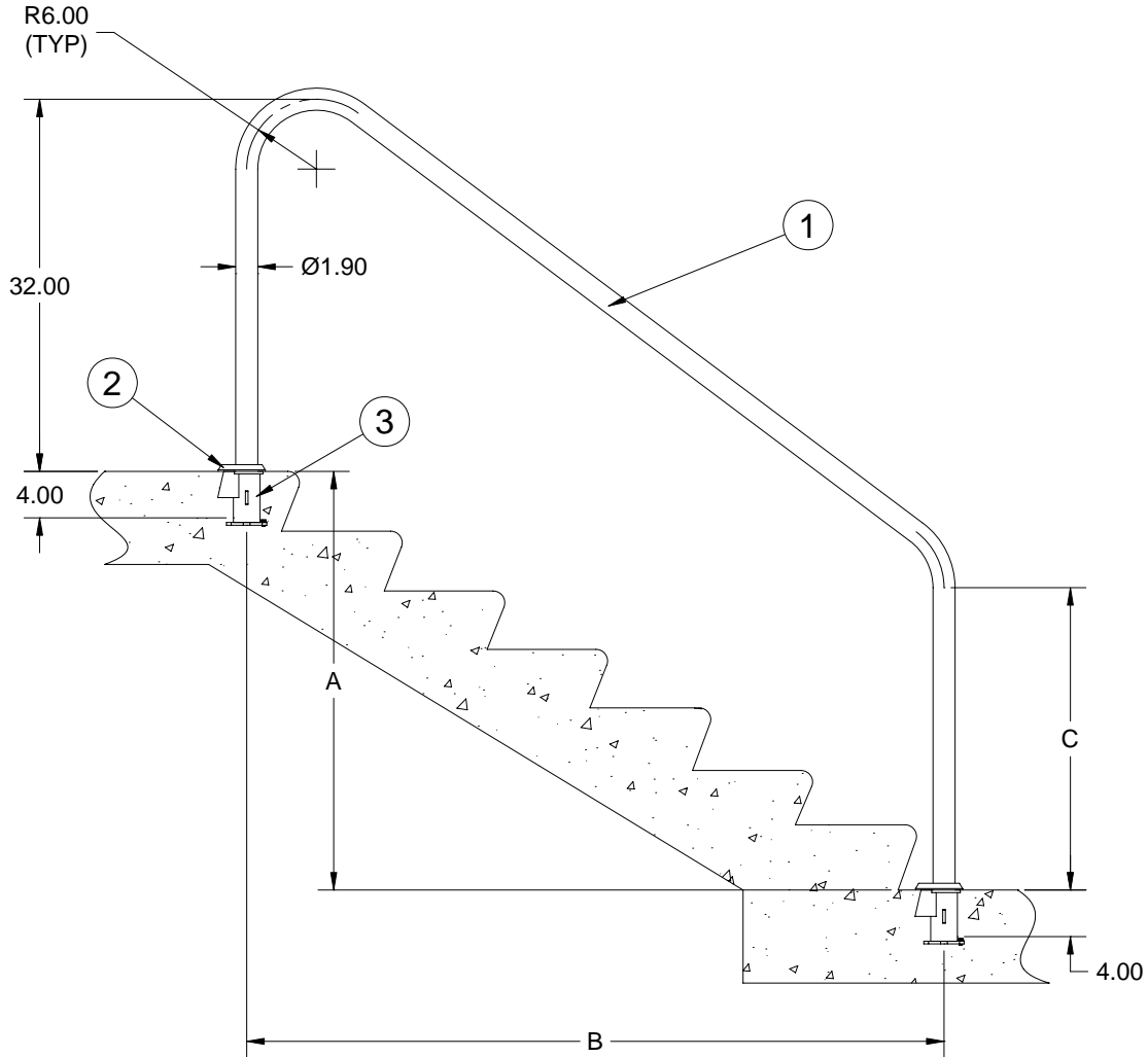
SIDE VIEW
