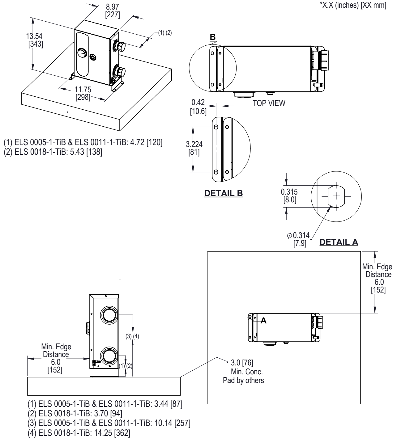
Figure 2. Hurricane Tie Down Details (2-Element Unit)
