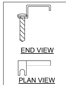
GRATING CLIP WITH SCREW FASTENING DETAIL
