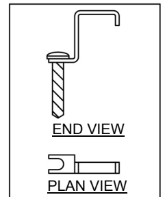
GRATING CLIP WITH SCREW FASTENING DETAIL
