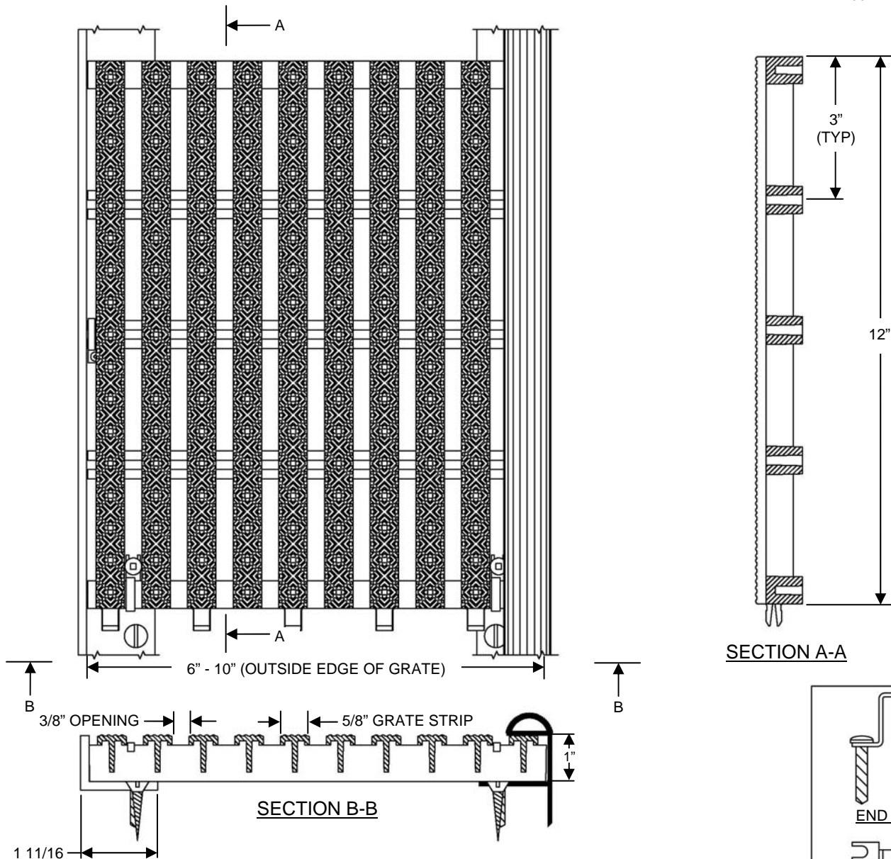
GRATING CLIP WITH SCREW FASTENING DETAIL
