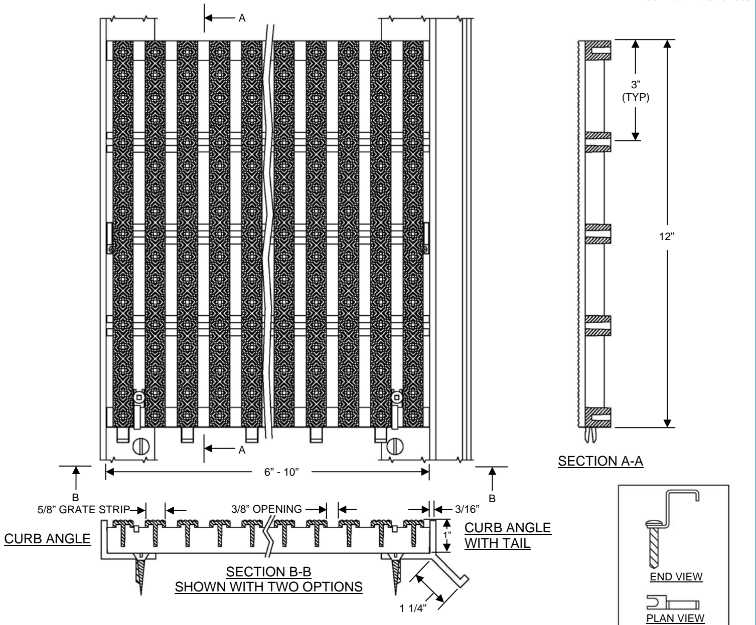
GRATING CLIP WITH SCREW FASTENING DETAIL
