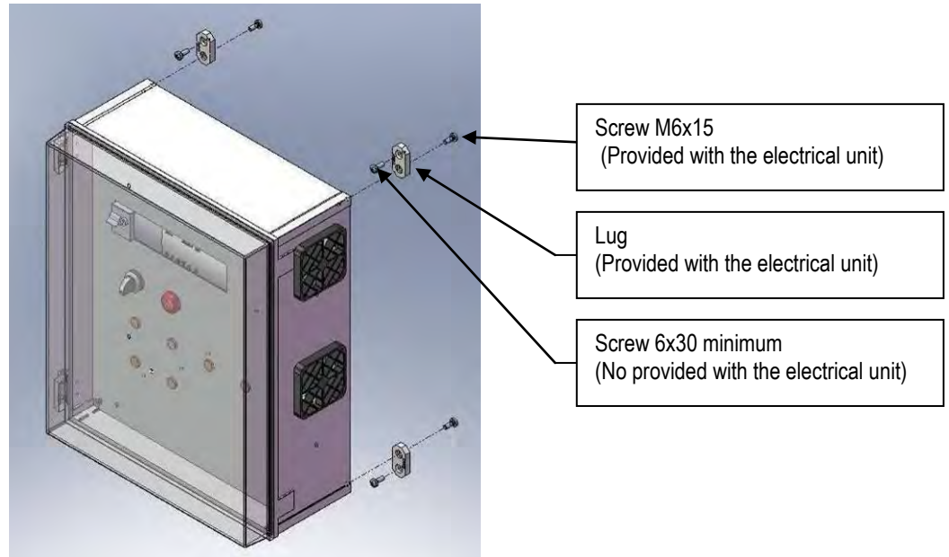
Diagram: fixing of electrical unit in the wall
