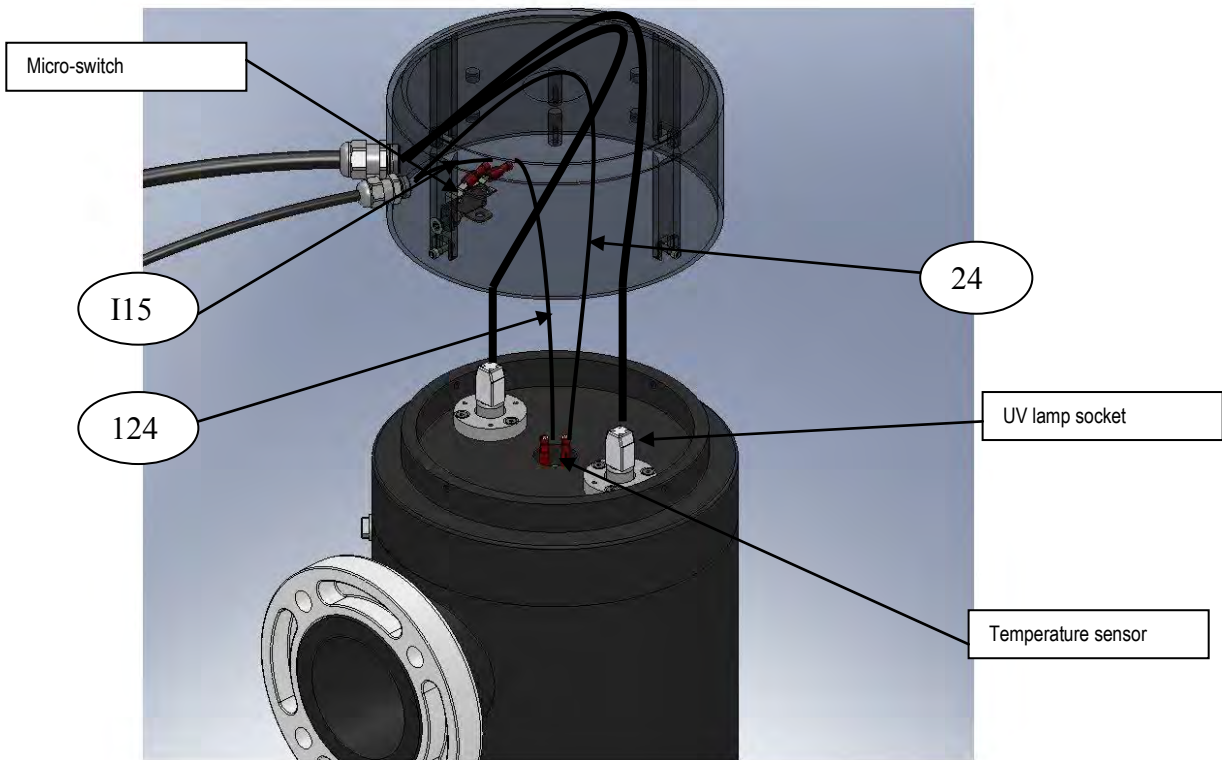
Diagram: Terminal connecting in the reactor
