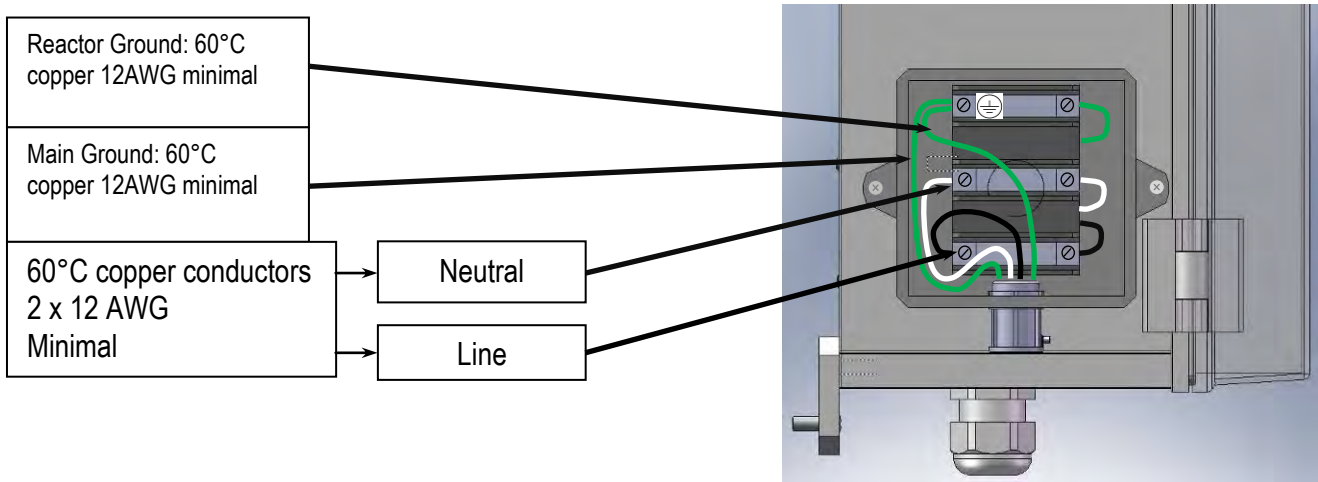
DIAGRAM: Wiring Terminal
