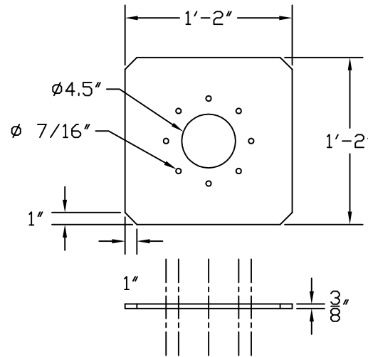
ANTI-VORTEX DETAIL SCALE: NTS
